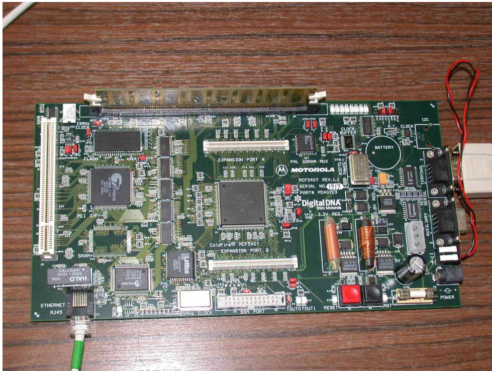
Figure 4 : Carte Motorola M5407C3
